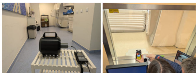
Figure 2. Experimental setup used during the practical sessions. Left: neutron survey meter used for radiation measurements in a radiotherapy facility. Right: Geiger-Müller survey meters used to measure ambient dose equivalent rate during shielding verification of a gamma camera room, simulating a routine clinical examination.
