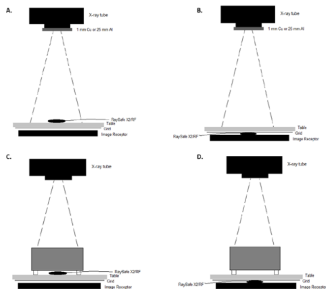
Figure 1. Experimental setups used for air kerma measurements under different conditions: A) 1 mm Cu or 25 mm Al, dosimeter on the table, with anti-scatter grid; B) 1 mm Cu or 25 mm Al, dosimeter on the image receptor, with anti-scatter grid. C) 20 cm PMMA, dosimeter on the table, with anti-scatter grid. D) 20 cm PMMA, dosimeter on the image receptor, with anti-scatter grid. All configurations were repeated without the anti-scatter grid.
