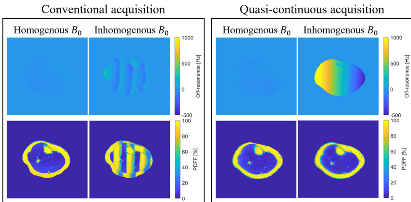
Figure 2. Comparison of conventional Dixon and quasi-continuous acquisitions under homogeneous and inhomogeneous B_0 conditions in the calf. Top: B_0 field maps; bottom: PDFF maps. Adapted from [5], licensed under CC BY 4.0.
