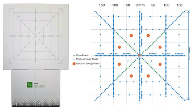
Figure 1. myQA StarTrack 3 detector on the left and a schematic view of the inner pixel distribution on the right.
